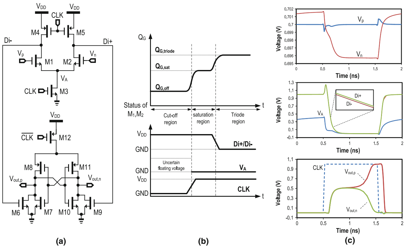
Fig. 2 a A conventional dynamic latched comparator. b The timing diagram shows the states and charge induced on the gate of M_1 ( M_2 ). c The simulated operation voltages of critical nodes
