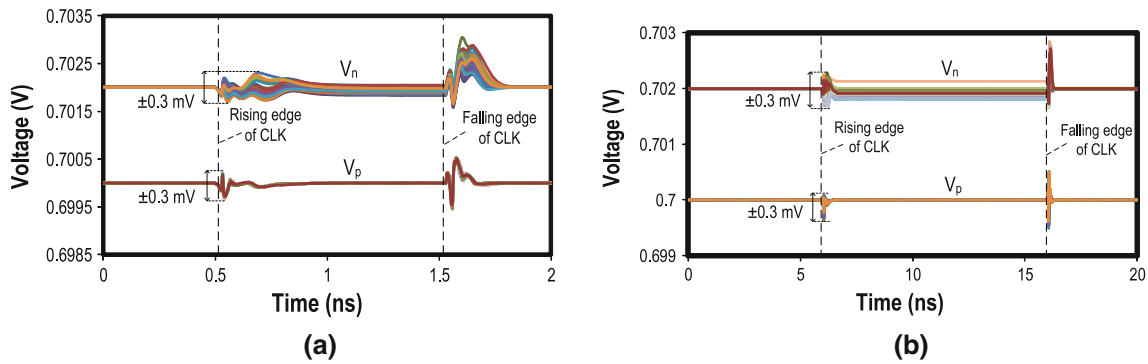
Fig. 5 Waveforms of proposed comparator’s V_n and V_p in 30 \times Monte–Carlo simulations. a f_{CLK} = 500 MHz, b f_{CLK} = 50 MHz
