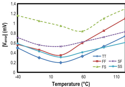
Fig. 6 Maximum deviation of the voltage on the capacitor at different temperature and process corners
