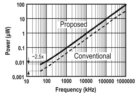
Fig. 8 Dynamic power versus the CLK frequency of the conventional and proposed comparators
