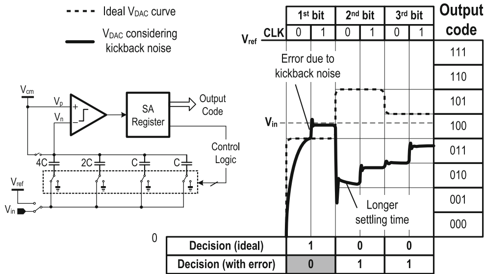
Fig. 1 SAR-type ADC with error code and longer settling time due to kickback noise
