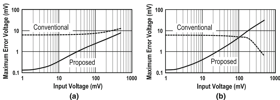
Fig. 4 Maximum input voltage variation due to kickback noise versus input voltage difference a V_n > V_p , b V_n < V_p
