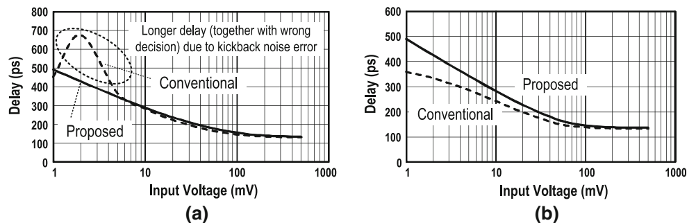
Fig. 7 Delay of the comparators versus input voltage difference in a V_n > V_p and b V_n < V_p cases
