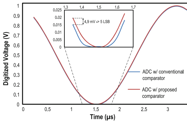
Fig. 9 Digitized waveform of a 1V_{pp} sinusoidal signal by two ADCs with conventional and proposed comparator
