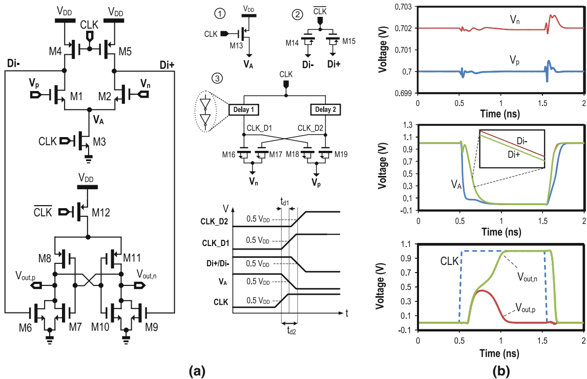
Fig. 3 a Proposed dynamic latched comparator with kickback-noise compensation. The extra elements are three sets of clocked NMOS-PMOS capacitors. b The simulated operation voltages of critical nodes
